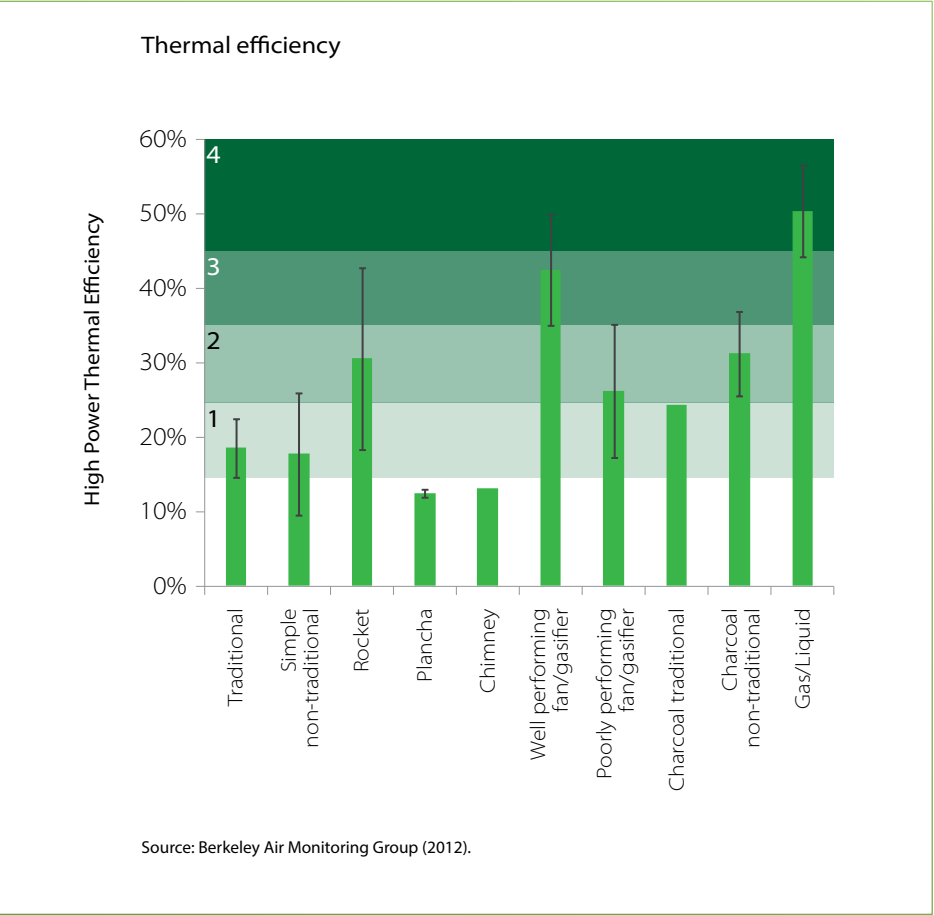
Figure 11.2: Technology comparison by thermal efficiency (WBT)
