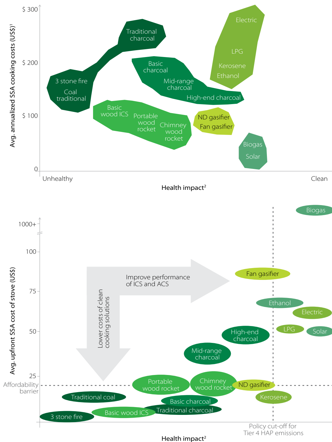
Figure 13: Relationship between cooking solution performance (HAP emissions) and cost
